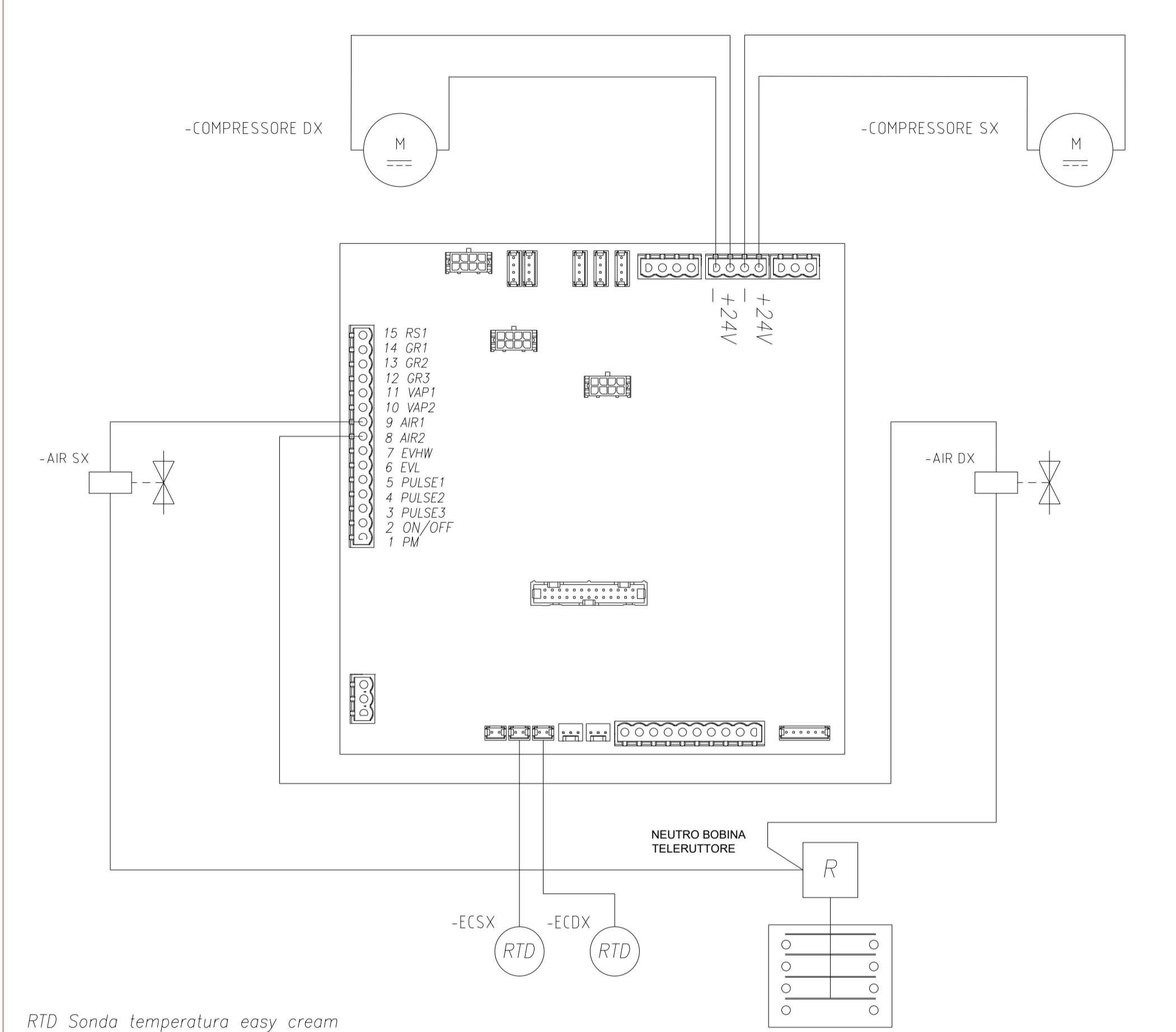
RTD Sonda temperatura easy cream
